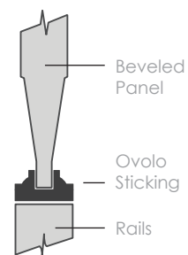
Beveled Panel with Ovolo Sticking
